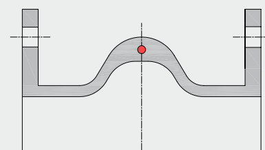
Vulcanised supporting ring (example)
